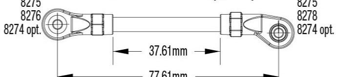
PANHARD BAR (QTY. 1)
