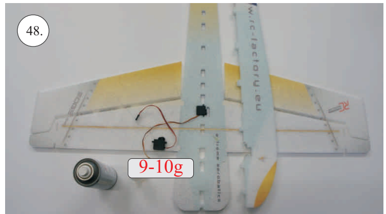
Aileron servo
