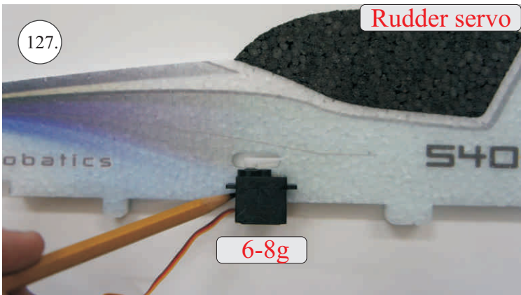
Rudder servo
