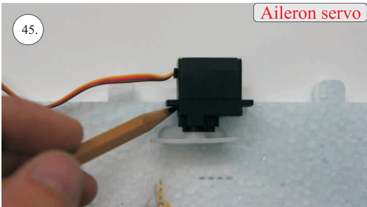
Aileron servo
