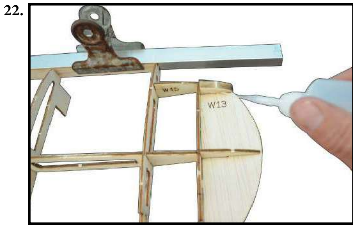
- Install W15 (6mm balsa wood) to wing and apply CA Glue to keep fixed as photo.
