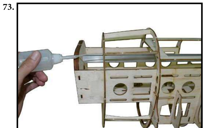
- Apply thin CA Glue around block include 2 layers former F2,F2'.
