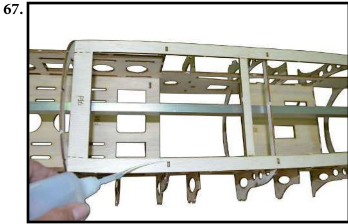
- Install F16 and apply CA Glue to keep fixed.
