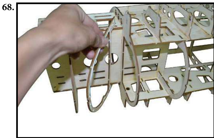
- Install F2' to F2 by White Glue.
