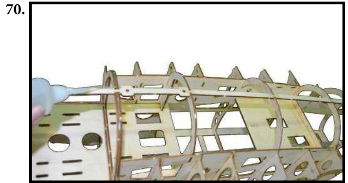
- Install F26 and apply CA Glue to keep fixed.
