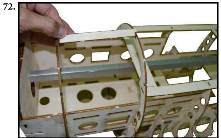
- Install F27 and apply CA Glue to keep fixed.
