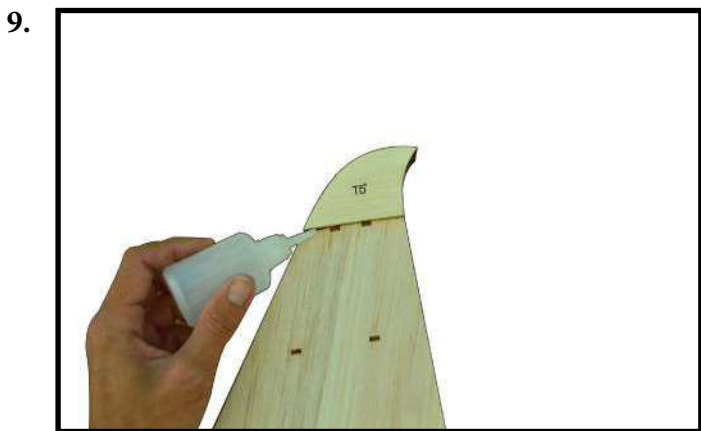
- Attach 8mm balsa block T5' by CA glue as photo.
