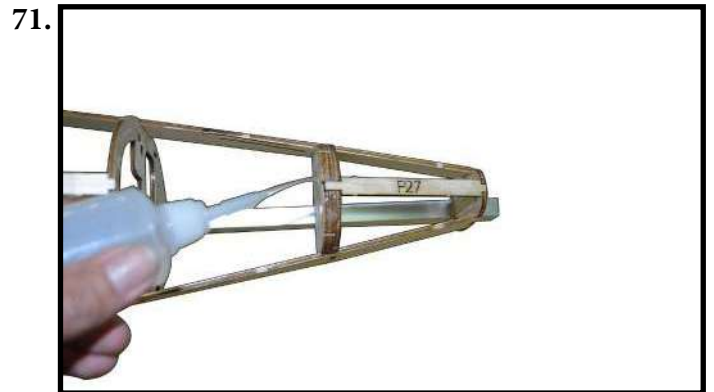
- Install F27 and apply CA Glue to keep fixed.
