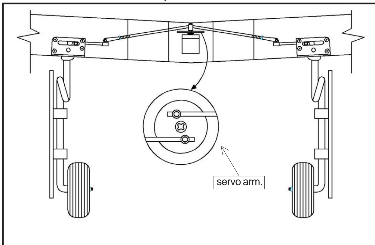
Open Position.
