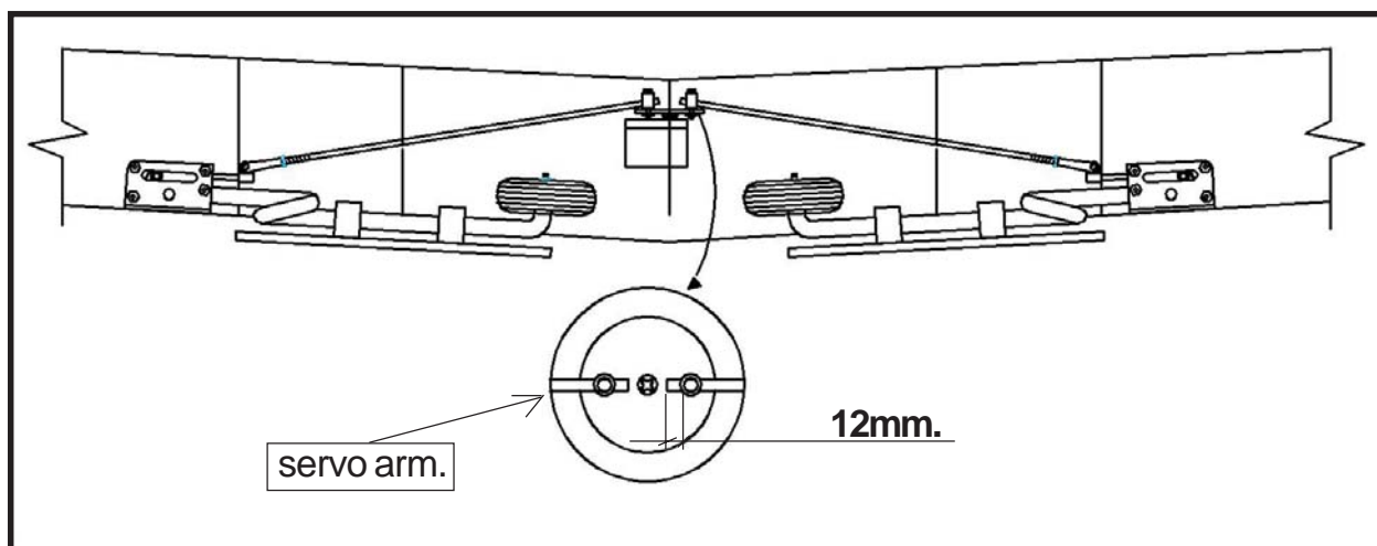
Close Position.
